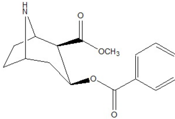
Norcocaine
