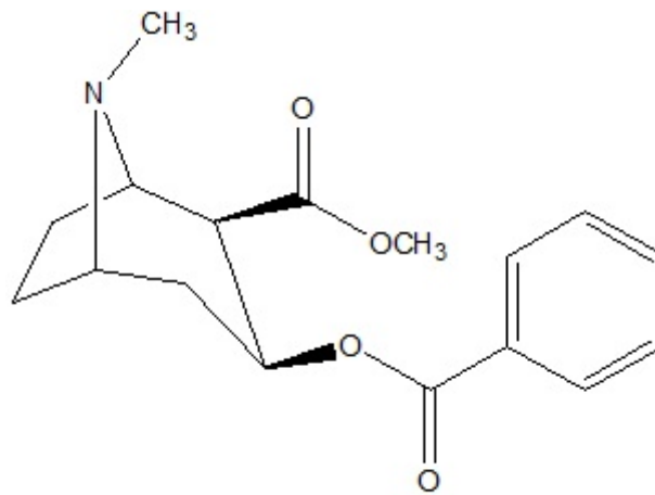
Cocaine
